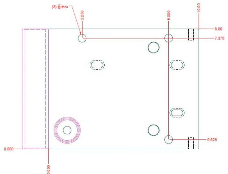
Top view of the PHP110-Ultra base, showing the mounting holes to attach the machine to a workbench or cleaning truck deck, and measurements below for mounting.
