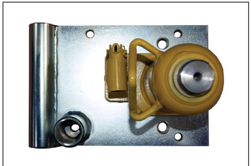
Top view of the PHP110-Ultra base, showing the mounting holes to attach the machine to a workbench or cleaning truck deck, and measurements below for mounting.
